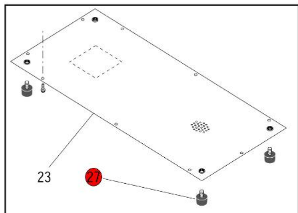
First Type-One Piece Floor With Adjustable Legs
