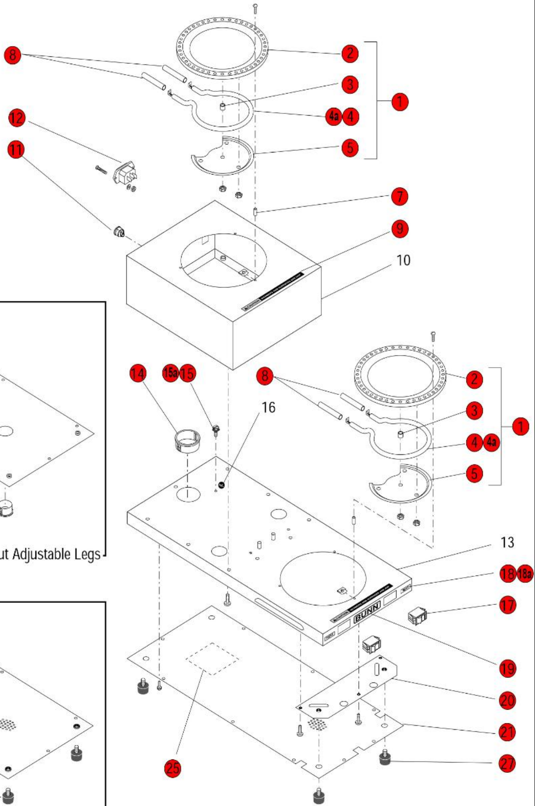
First Type-One Piece Floor With Adjustable Legs
