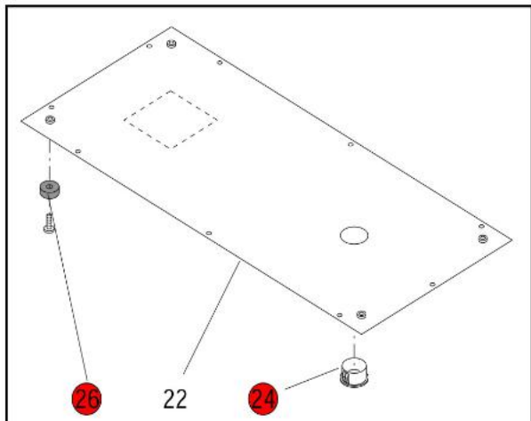
First Type-One Piece Floor Without Adjustable Legs
