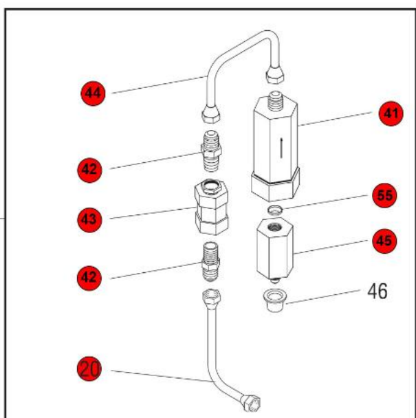
Optional - Quiet Strainer/Flow Control
