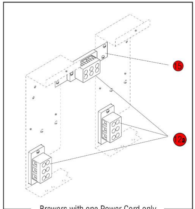
Brewers with one Power Cord only
