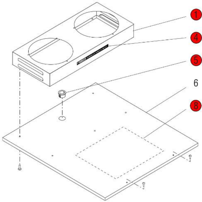
2/2 W/TOP WARMERS (REAR)
