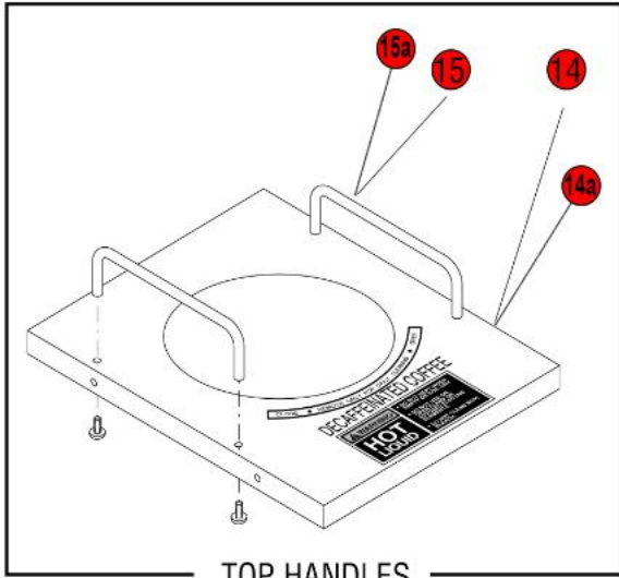
TOP HANDLES
